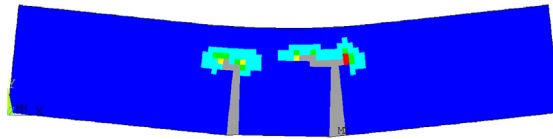
Fig. 19. Maximum principal strain contour of final crack pattern by SLA for the 5 MPa prestress test.
