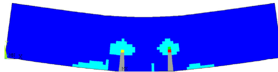
Fig. 23. Maximum principal strain contour of the final crack pattern of SLA for the 10 MPa prestress.
