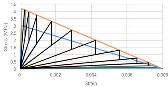
Fig. 10. Stiffness reduction procedure: sequentially reduced stiffness to 50% of the previous value.
