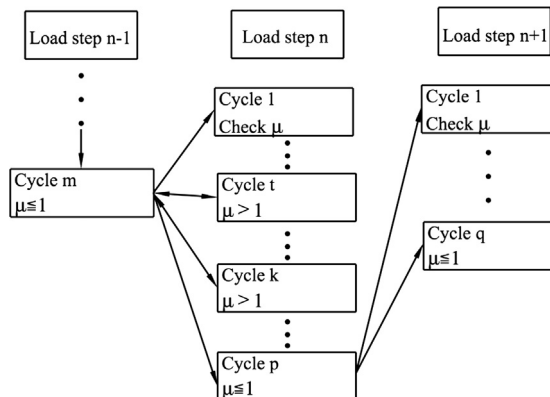
Fig. 5. Restart procedure of the algorithm.
