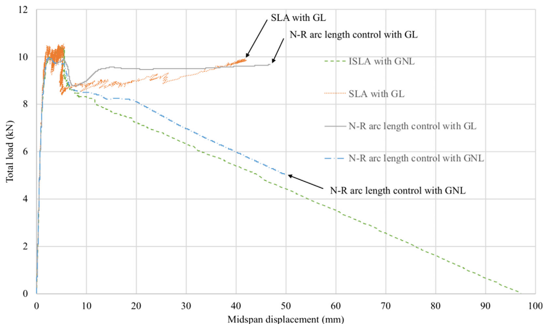
Fig. 28. Midspan displacement-force curves for comparison of geometrical linear and non-linear effects.
