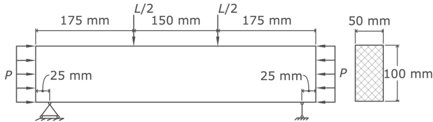
Fig. 8. Test model dimension and load combination.
