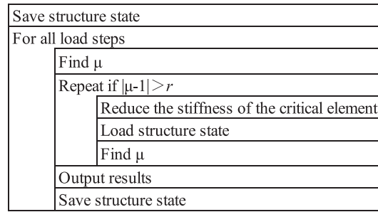
Fig. 2. Program structure diagram for the Load control.
