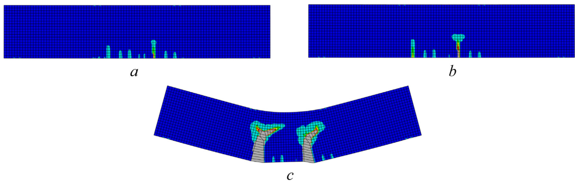
Fig. 21. Maximum principal strain contours of the crack propagation of the N-R arc length control analysis for the 5 MPa prestress.
