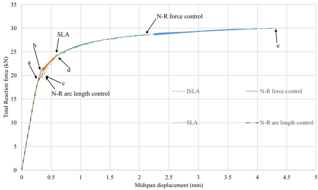
Fig. 22. Reaction force-displacement diagram for the 10 MPa prestress.
