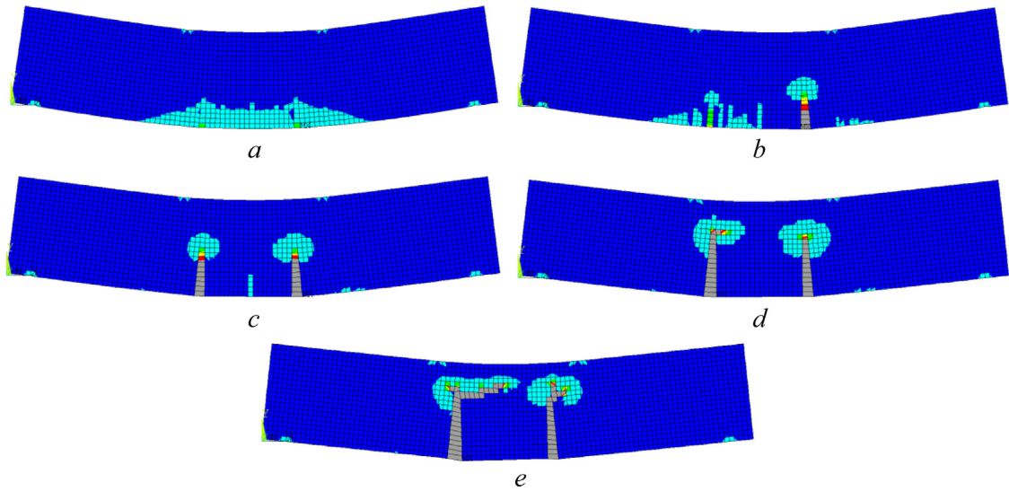
Fig. 18. Maximum principal strain contours of crack propagation by the proposed method for the 5 MPa prestress test.
