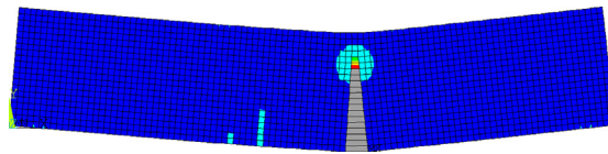
Fig. 13. Maximum principal strain contour when the midspan displacement is 0.3 mm by the proposed method for the 1 MPa prestress test.
