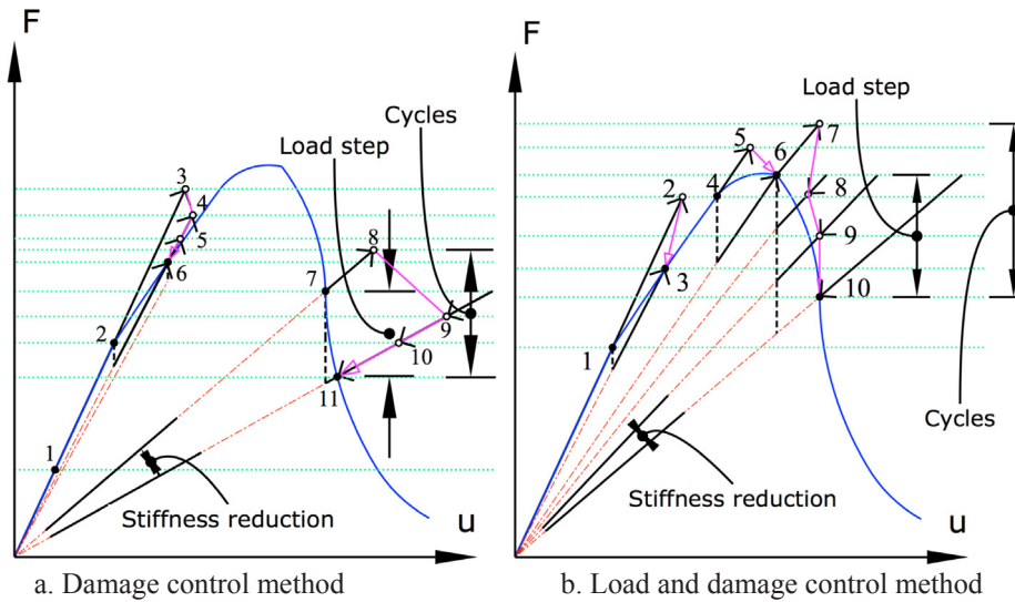
Fig. 7. Searching path of Load scaling control.
