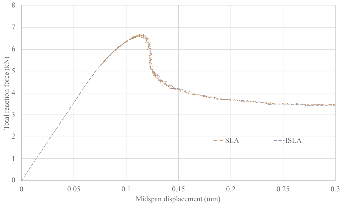
Fig. 12. Reaction force-displacement diagrams for the 1 MPa prestress test.
