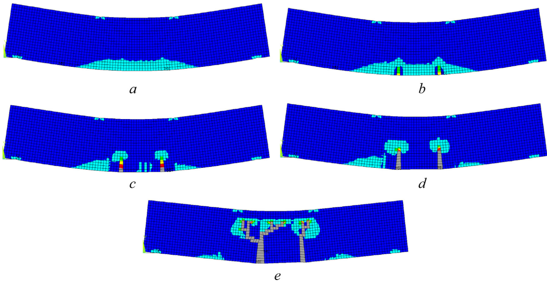
Fig. 24. Maximum principal strain contours of the crack propagation of the proposed method for the 10 MPa prestress.
