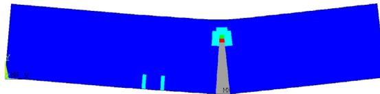
Fig. 14. Maximum principal strain contour when the midspan displacement is 0.3 mm by SLA for the 1 MPa prestress test.
