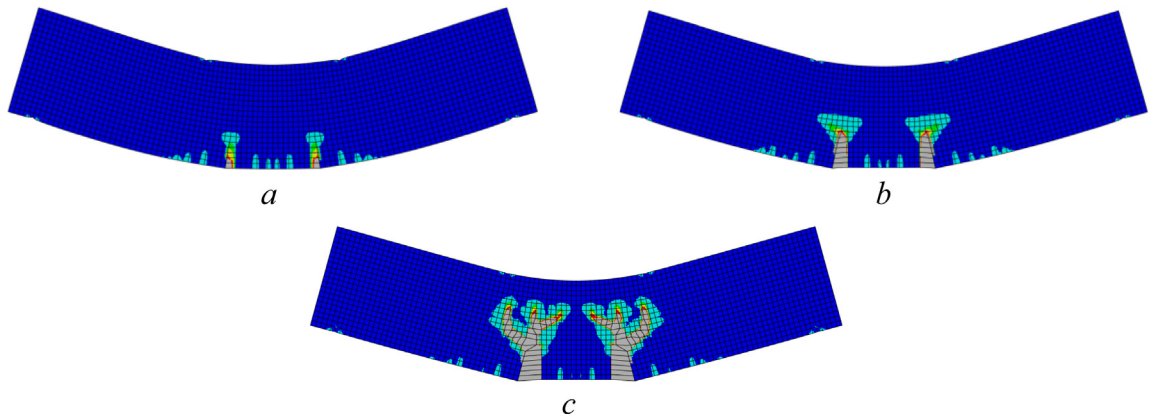
Fig. 25. Maximum principal strain contours of the crack propagation by N-R force control for the 10 MPa prestress.
