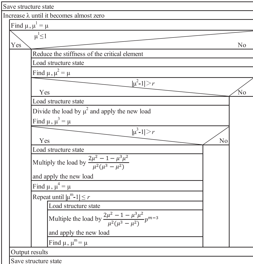
Fig. 4. Program structure diagram of the Damage control method in Load scaling control.
