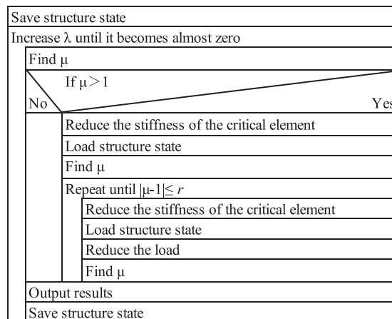
Fig. 6. Program structure diagram of Load and damage control method in Load scaling control.
