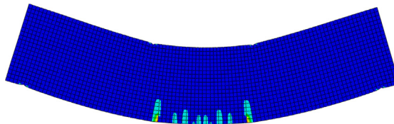
Fig. 20. Maximum principal strain contour of final crack pattern by N-R force control analysis for the 5 MPa prestress test.
