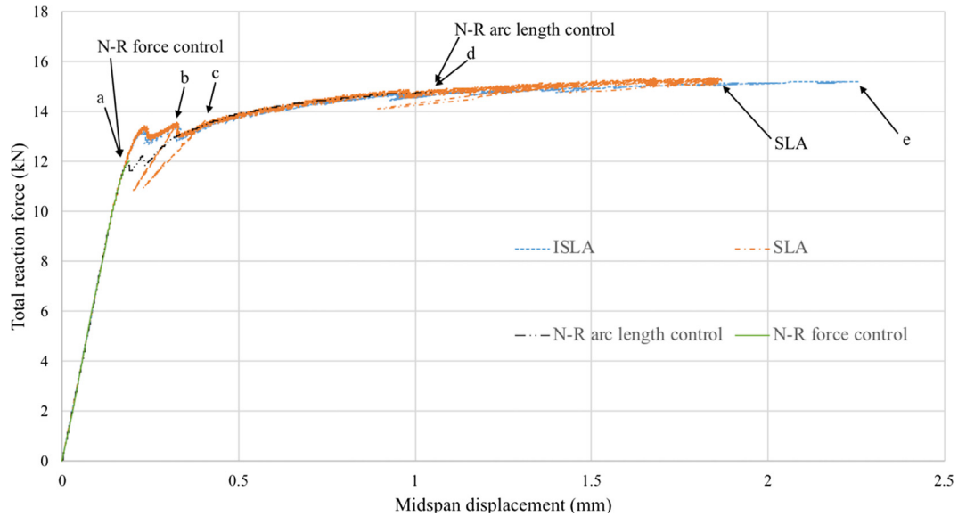
Fig. 15. Reaction force-displacement diagrams for the 5 MPa prestress test.
