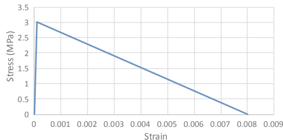
Fig. 9. Material properties of concrete (tension softening).
