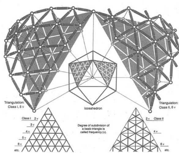
Figure C.6: Subdividing the faces according to class I and II, from (Wester 1984).
