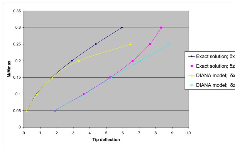
Figure 7.11: The differences between DIANA and the exact solution for the bending benchmark
