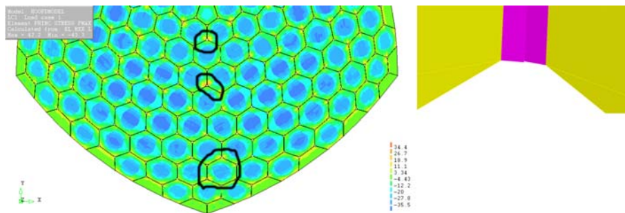
Figure 4.16: Left: Deviation in the connection of the kinked joint; also note the difference in the angles of the edges. Right: small deviations peaks in the stress distribution that are possibly arising from this geometry.
