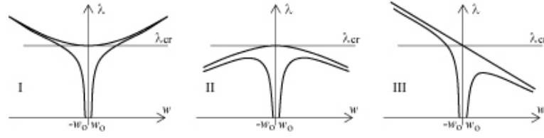
Figure B.7: Basic types of post buckling behaviour (Koiter 1945).
