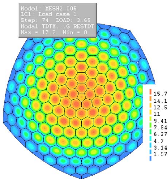
Figure 7.3: The results for the dome with a finer (2x) mesh; max. deflection at \lambda = 3.65 :17.2mm
