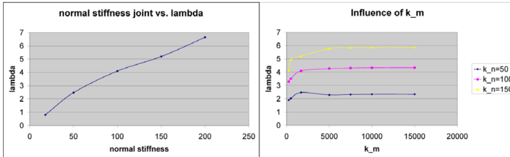
Figure 4: The influence of the normal stiffness ( k_n ) and the bending stiffness ( k_m ) on the buckling factor of the structure.
