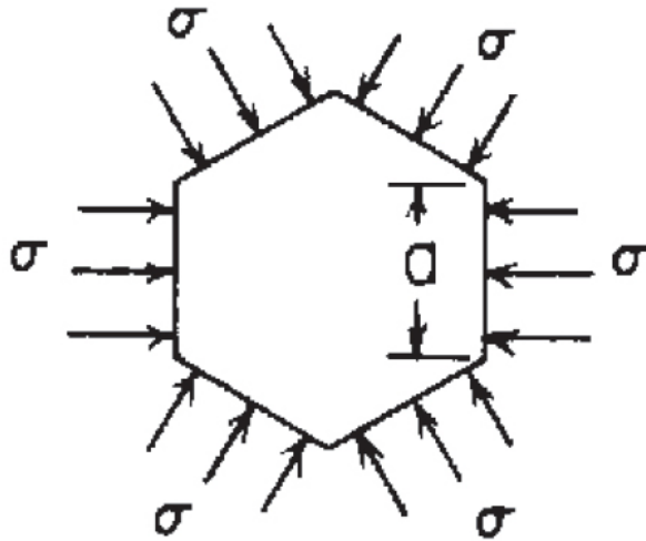
Figure 9.1: Scheme of a polygon plate under uniform compression on all edges, from (Young & Budynas 2001).
