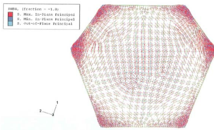
Figure 3.6: The stresses in a corner of a plate; simply supported plate with a evenly distributed load of 1,0 \text{ kN/m}^2 perpendicular to the plane. From (Isgreen 2007).
