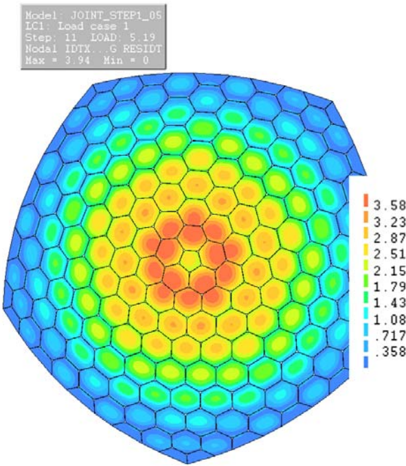
Figure 12.6: The results of Model I (last incremental deformation is shown).
