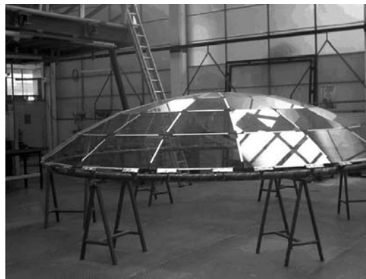
Figure 2.4: The facettted glass dome developed at the Delft University of Technology, from (Veer et al. 2003).
