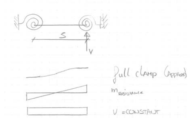
Figure H.13: Scheme of the connection between the bending stresses and the shear stiffness.
