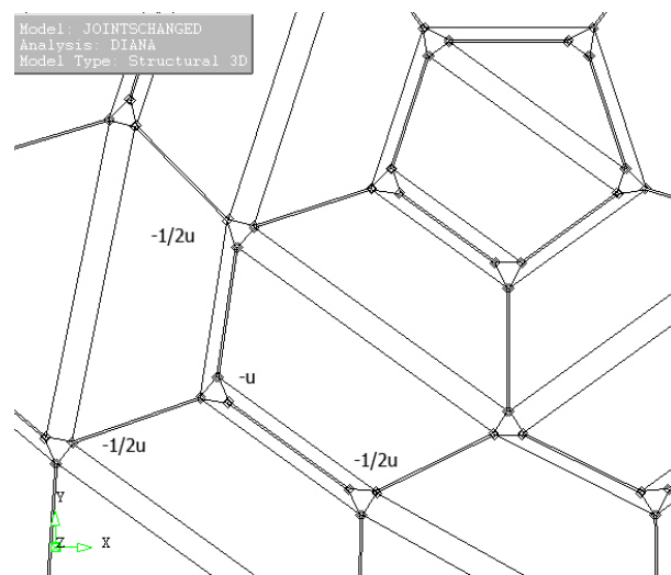
Figure 10.3: Zoomed in on the dome; corner of the first hexagon: one node will be displaced maximally, while three nodes will be displaced half way. In every node six points will be displaced equally.
