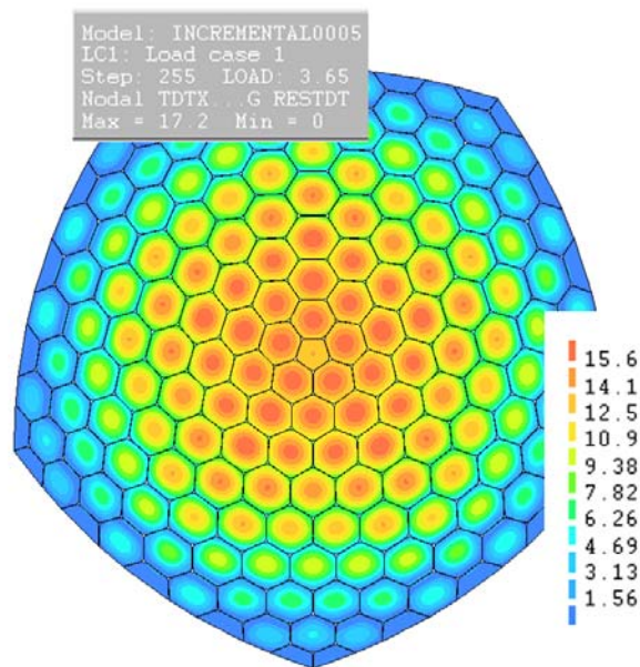
Figure 7.2: The results for the dome with the original mesh; max. deflection at \lambda = 3.65 :17.2mm.
