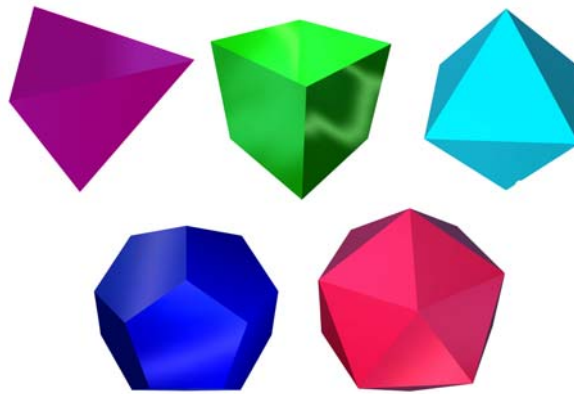
Figure C.7: The five regular platonic solids, from ( 2007j).
