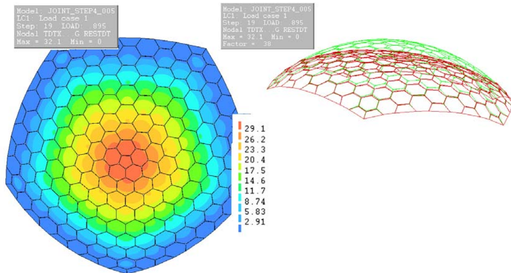
Figure 12.5: The results for combination 3: d = 36,5mm and E_j = 2,43MPa
