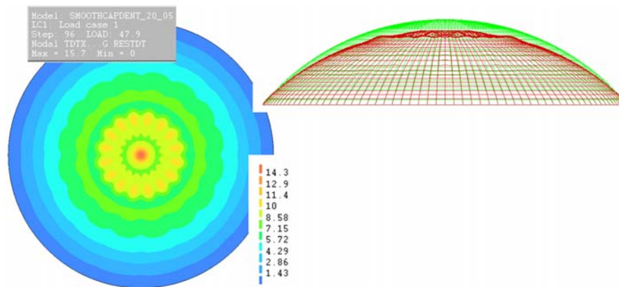
Figure 12.19: The result of the buckling calculation for a smooth glass dome with an imperfect geometry.
