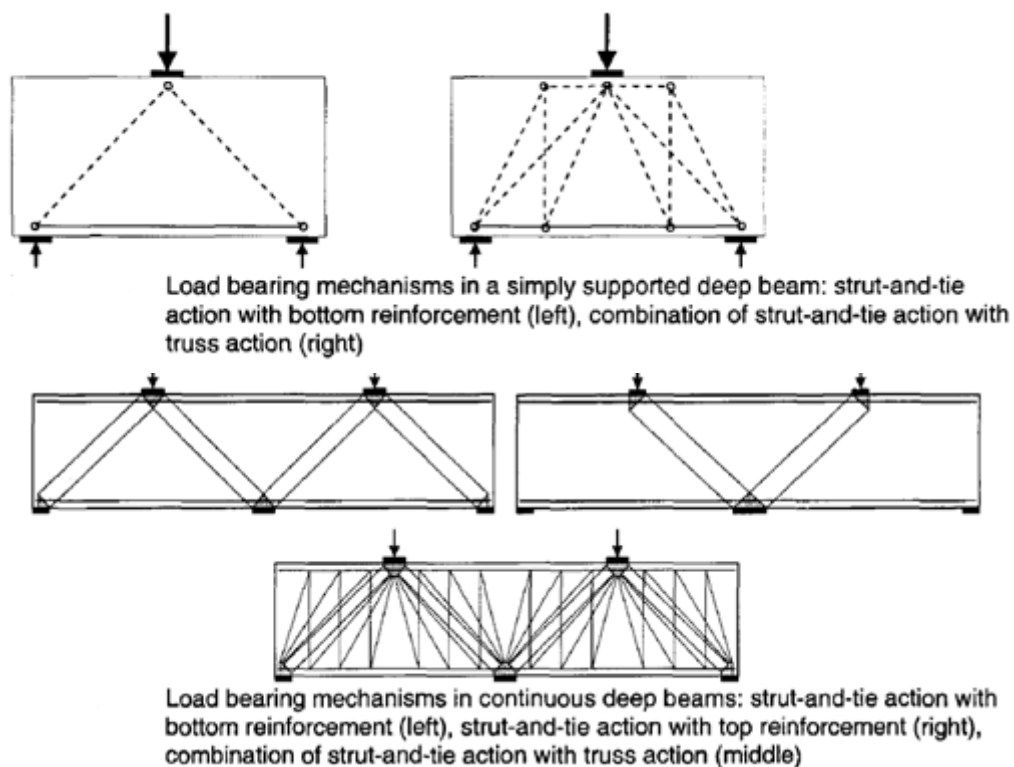
Figure 1.11 Load bearing mechanisms [3]
