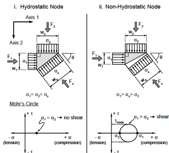
Figure 2.7 Mechanics of hydrostatic and non-hydrostatic nodes [15]
