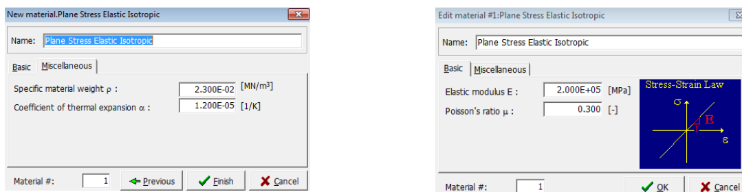
Figure 6.12 ATENA interface about the steel plate material property.
