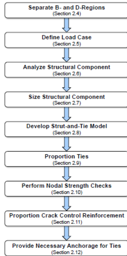
Figure 2.14 STM tree diagram[13]
