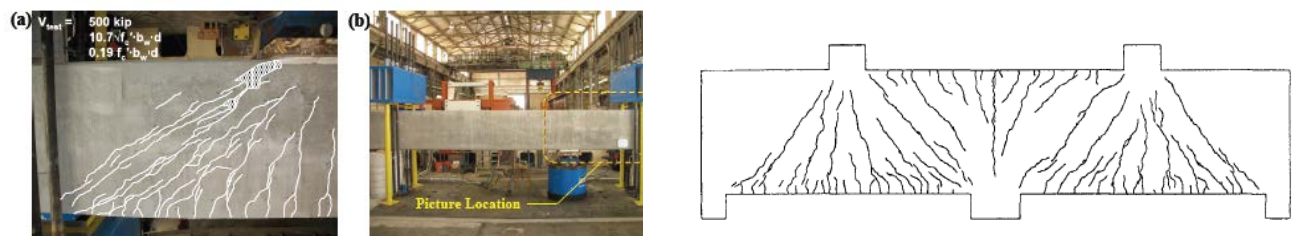
Figure 9.4 the cracking behavior of deep beam specimens
