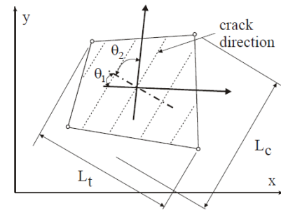
Figure 6.8 Definition of localization bands
