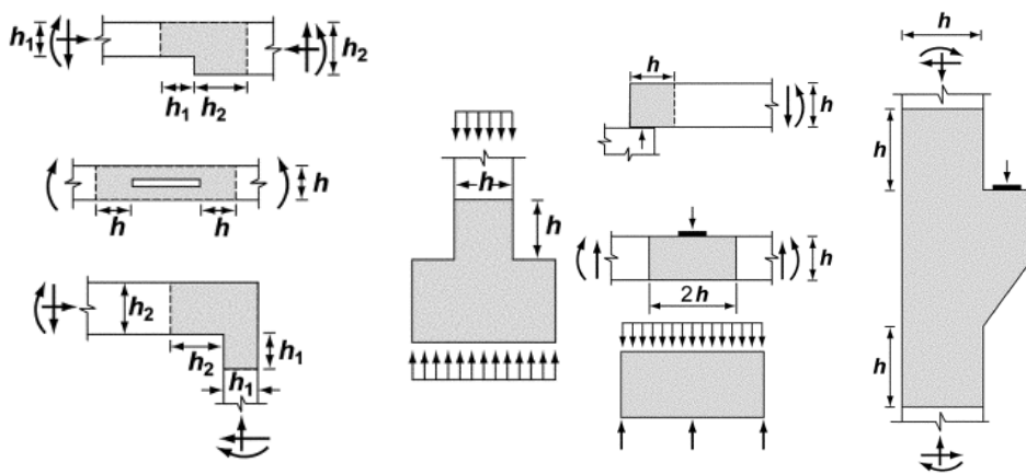
Figure 2.4 Loading and geometric discontinuities [18]
