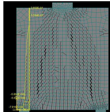
Figure 10.7 shear stresses near by support area
