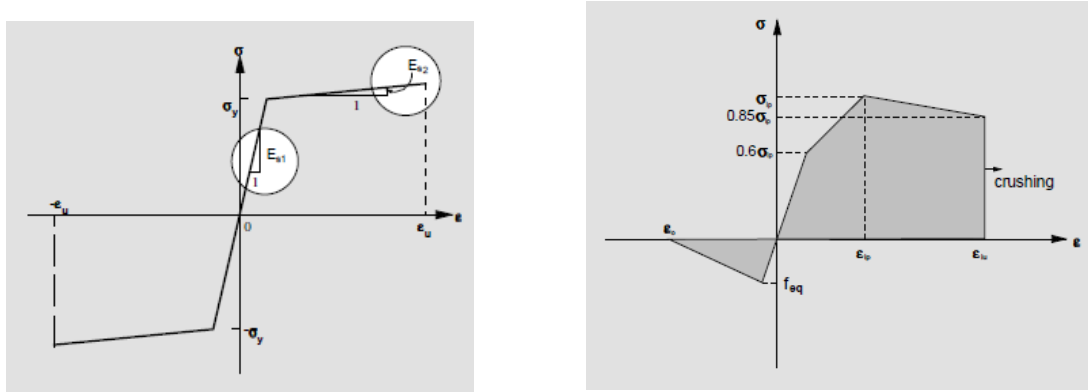
Figure 1.14 Steel stress-strain relation (left) and stress-strain relation for concrete (right)
