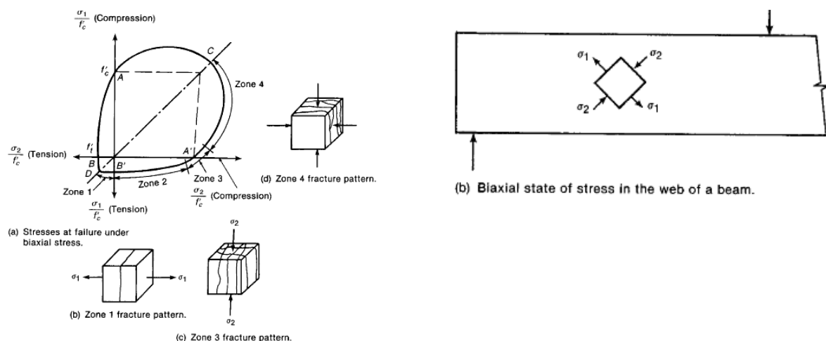
Figure 3.7 Strength and modes of failure of uncracked unreinforced concrete subjected to biaxial stresses (left) and the biaxial state of stress in the web of a beam (right)
