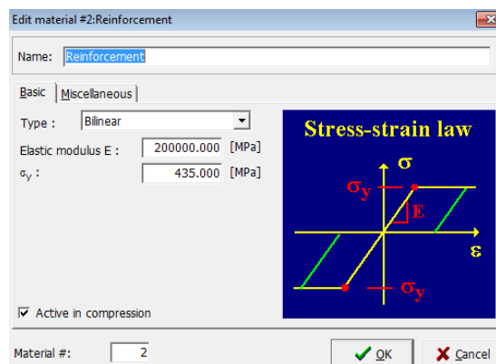
Figure 6.14 Reinforcement material properties in the ATENA interface
