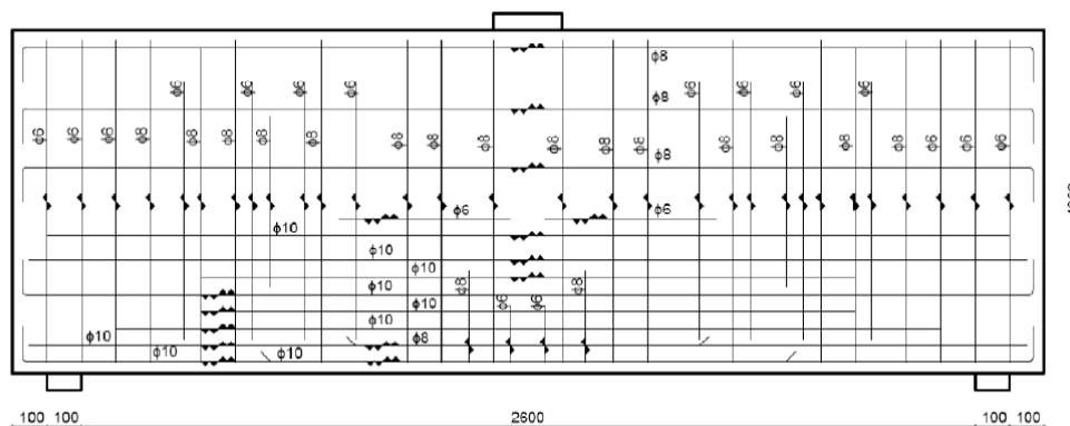
Figure 7.1 Reinforcement configurations [1], [2]
