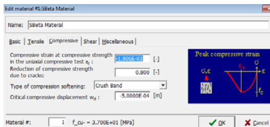
Figure 6.5 Compression strain
