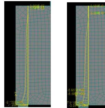
Figure 10.9 D1 specimen in ULS design (left) and in Failure ATENA (right)
