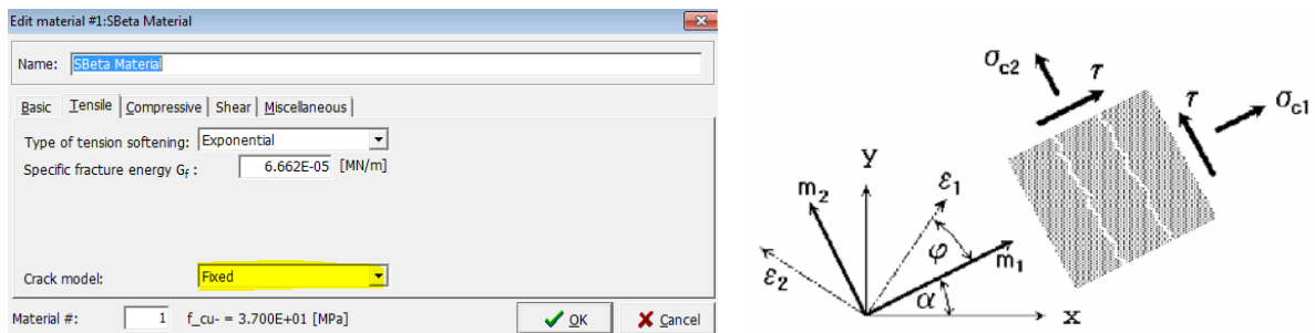
Figure 6.11 SBETA material model properties in ATENA software (left) and fixed crack model “Stress and strain state” (right)
