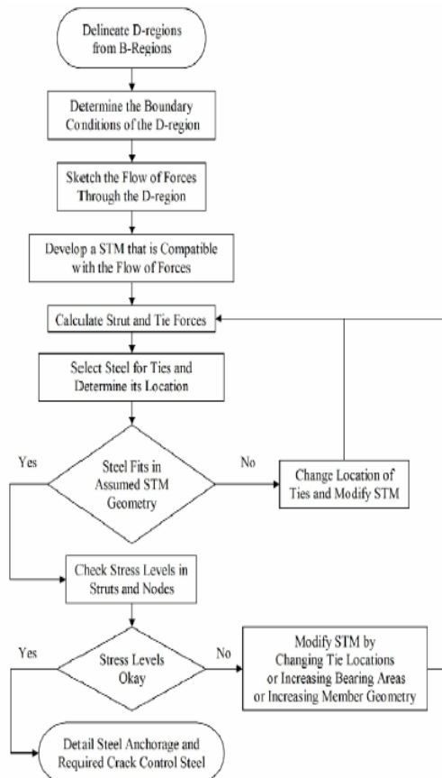
Figure 2.13 STM tree diagram [15]
