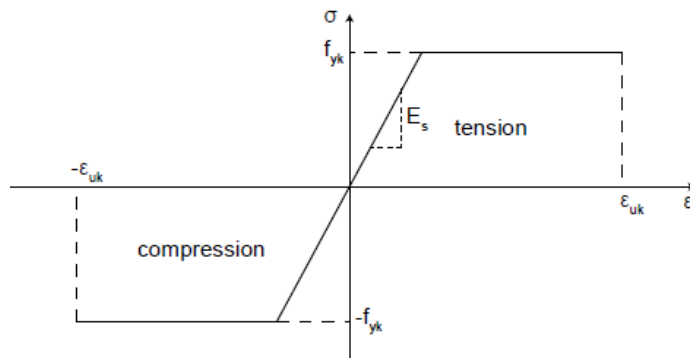
Figure 6.13 Stress-strain diagram
