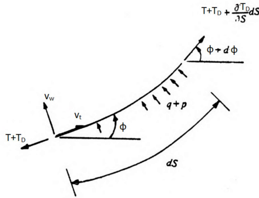
Figure D.10: equilibrium of element by dynamic forcing (adjusted [62])
