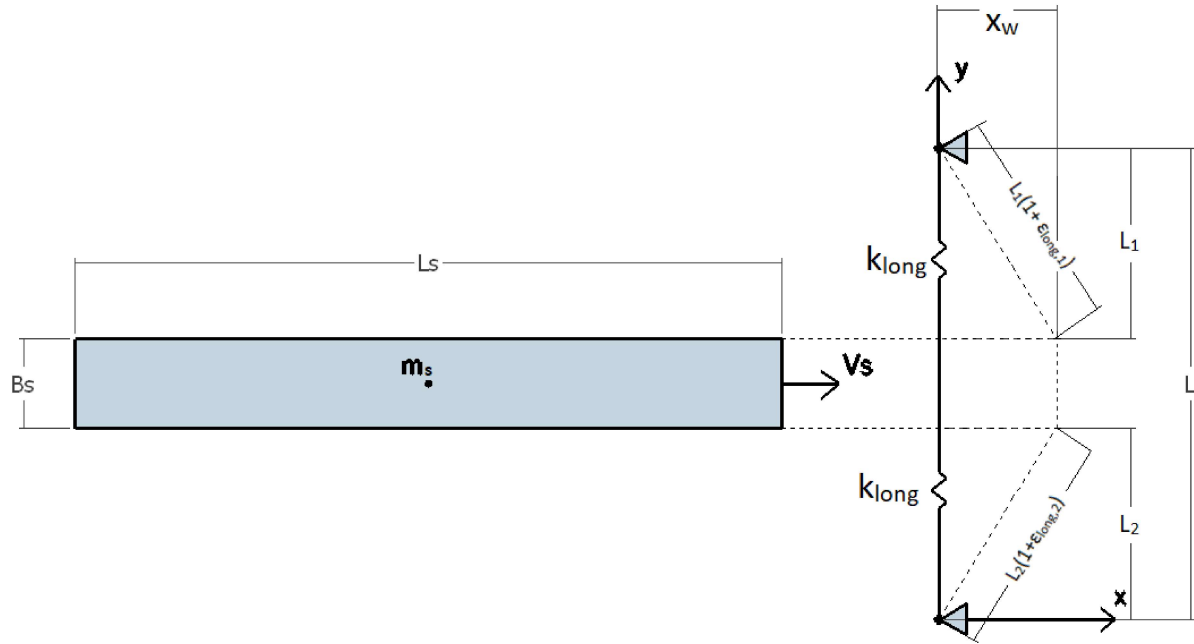
Figure 4.3: ship collision model top view
