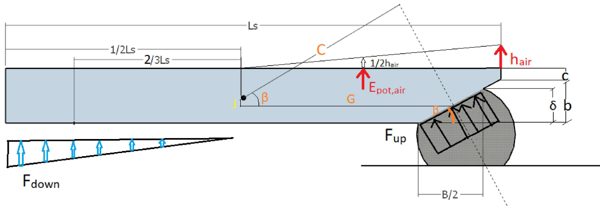
Figure 7.4: forces and moment static
