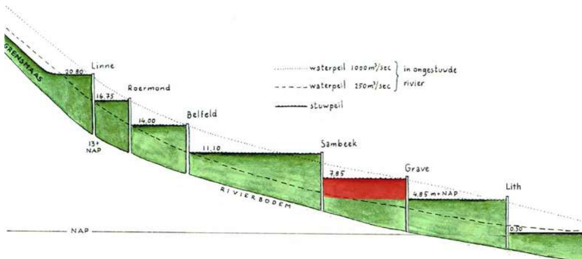
Figure 1.1: side view weirs in the Meuse [46]
