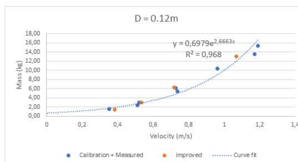
Figure 6.10: calibration 0.12 m
