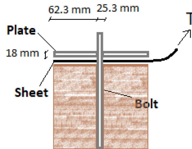
Figure 7.11: clamping dimensions
