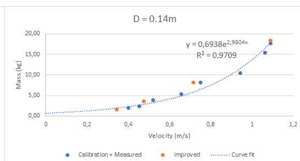
Figure 6.11: calibration 0.14 m
