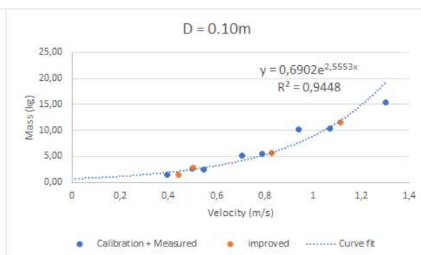
Figure 6.9: calibration 0.10 m
