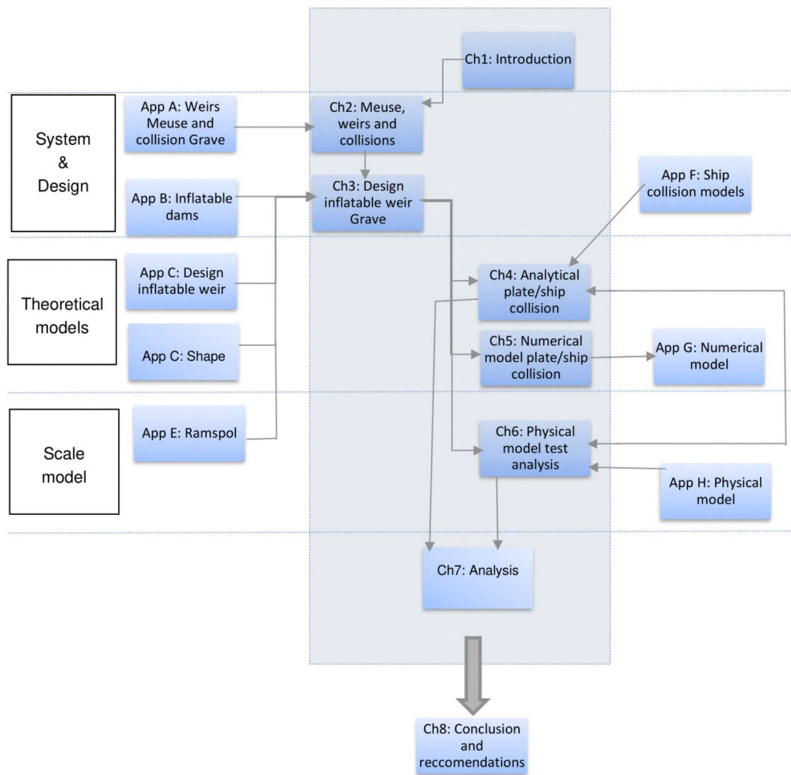
Figure 1.4: flowchart
