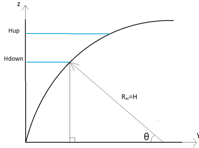
Figure C.7: geometry circular abutment
