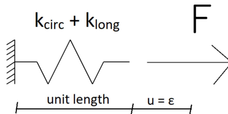
Figure 4.6: 1D-model
