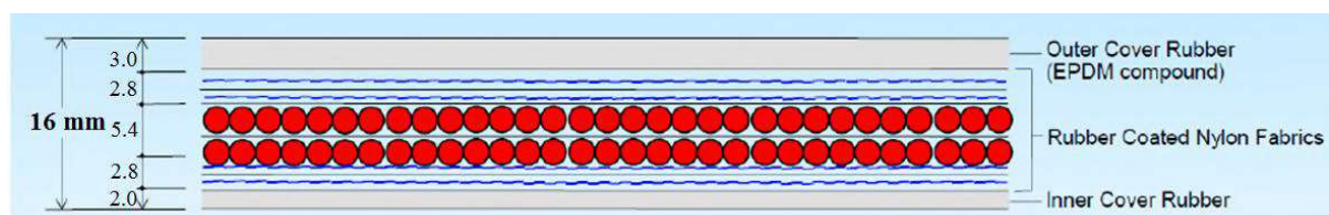
Figure 3.17: sheet cross section [5]
