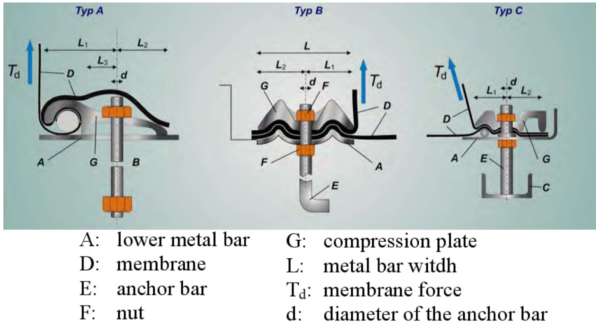
Figure C.6: three different clamping systems [65]
