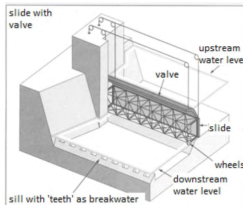
Figure 2.9: wheel valve [29]
