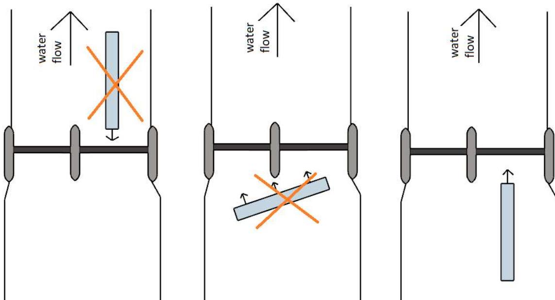
Figure 4.1: collision scenarios
