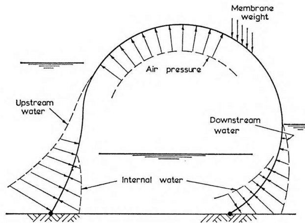
Figure 3.7: force overview [17]
