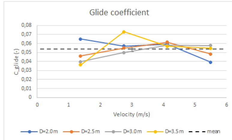
Figure 7.7: glide coefficient
