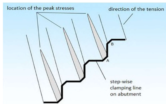
Figure E.4: stepwise clamping with abutments [38]
