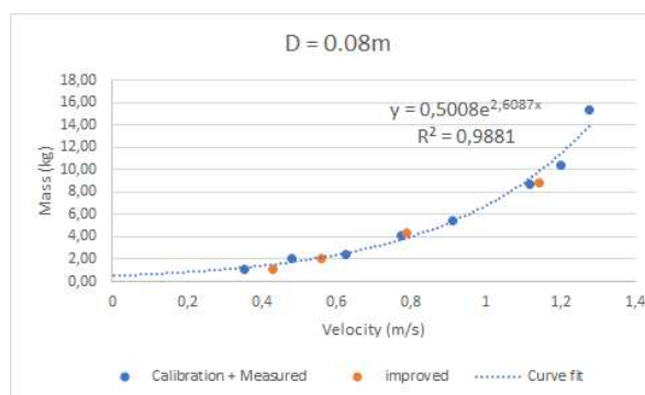
Figure 6.8: calibration 0.08 m
